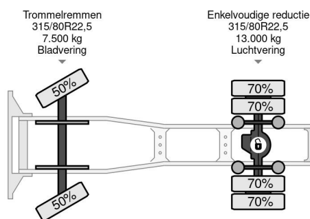
DAF 95.380 XF SPACECAB (EURO 2 / ZF16 MANUAL ... 4x2
