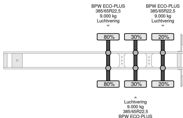
Magyar SITE P30P1A3 3-AXLE 1 COMPARTMENT 30.000 L... Referenznummer: SN 61014128
