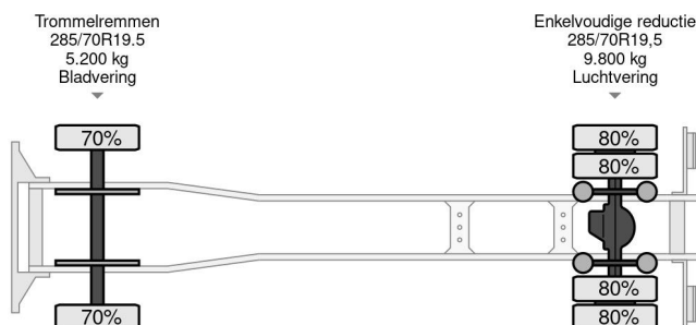
MAN F 15.192 (6-CILINDER) WITH GEESINK VACUUM... 4x2
