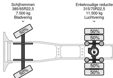
Renault Premium 450 DXI ALLIANCE HIGH ROOF (ZF... 4x2
