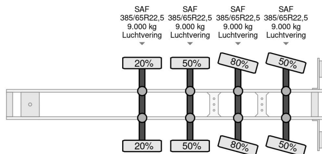
KWB KWB P-504-STI-H 4-AXLE FLATBED TRAILER (SAF A...
