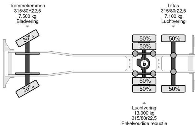
DAF 95.480 XF SPACECAB 6x2 WITH HOOK-ARM SYSTEM...
