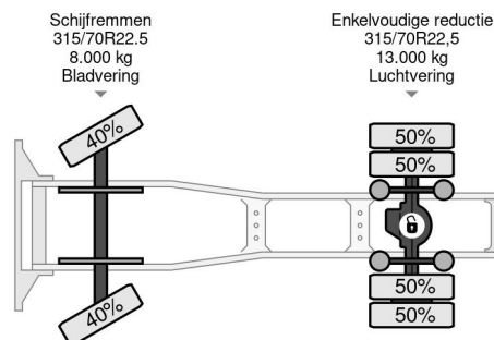
DAF XF 460 SUPERSPACECAB (ZF MANUAL GEARBOX / MX-BRAKE / 8.000 KG. FRONT AXLE / 995+500 LITER TANK / FRIDGE UNDER BED / ETC.) 4x2 Referentienummer: SN 60766372
