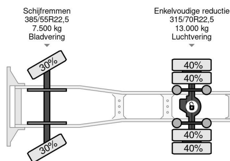
DAF XF 95.430 SPACECAB (EURO 4 / AS-TRONIC / F... 4x2
