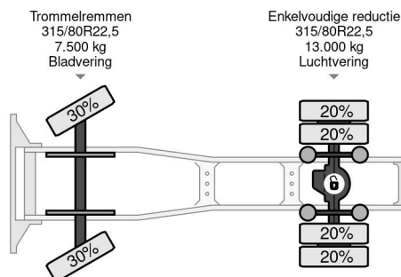
DAF 95.380 XF SPACECAB (EURO 2 (MECHANICAL ... 4x2 Referentienummer: SN 56068266 Z
