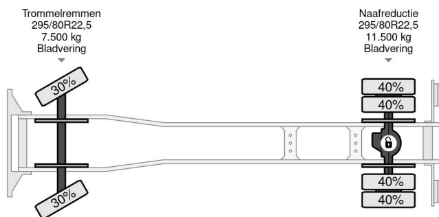
MAN 18 18.232 4x2 FULL STEEL CHASSIS (MANUAL GEA...
