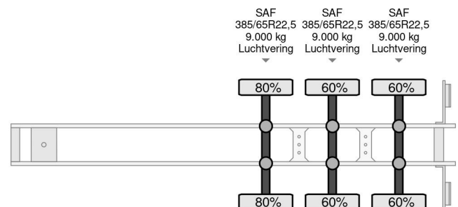
Pacton T3-001 13.60 METER (CURTAINSIDE) TRAILERPAC... Referentienummer: SN 54996280
